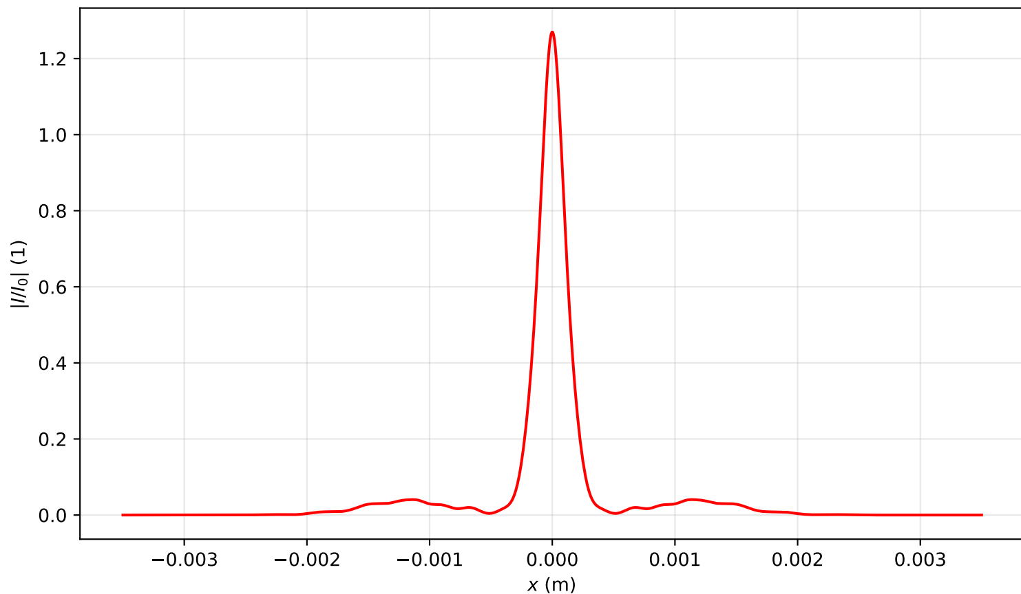
Intensity profile I(x, y = 0, z = 3.105)/I_0 , P_{in}=8.0P_{cr} , artificial time
